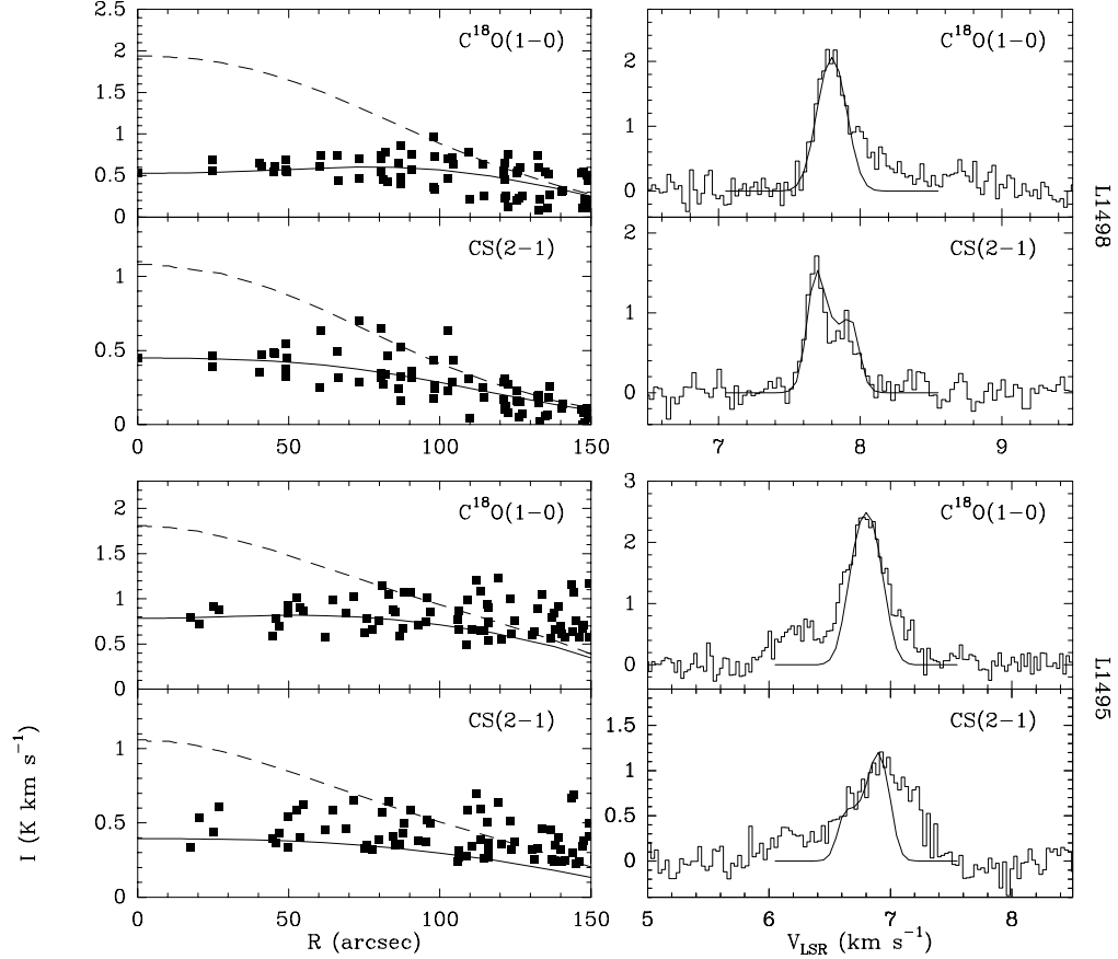
FIG. 3A.— Radial profiles of integrated emission (left) and central emerging spectrum (right) for \text{C}^{18}\text{O}(1-0) and \text{CS}(2-1) in each of our cores. Observations are indicated by solid squares in the radial profiles and by histograms in the spectra (all temperature units are in the main beam scale). The results from two radiative transfer models are plotted over the radial profiles: the dashed lines are constant abundance models and the solid lines are models with a rapid decrease in the central abundance. (Constant abundance models assume X(\text{C}^{18}\text{O}) = 1.3 \cdot 10^{-7} in all cores and X(\text{CS}) = 3.0 \cdot 10^{-9} in L1495 and L1517B, 2.0 \cdot 10^{-9} in L1498 and L1544, and 6.0 \cdot 10^{-9} in L1400K. See Table 4 for parameters of the models with a central abundance drop.) Note how the constant abundance models fail to fit the central emission, while the models with variable abundance fit the data at all radii satisfactorily. The predicted emerging intensities of these variable abundance models (after convolution) are presented by solid lines overlaid on the central spectra in the right panels. Note the presence of additional velocity components in the \text{C}^{18}\text{O} emission toward L1498 and in \text{C}^{18}\text{O} and \text{CS} toward L1495. These components probably arise from unrelated ambient gas and have not been included in the integrated emission of the radial profiles.
